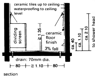
⑥ Shower room
